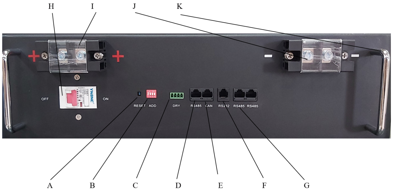
Figure 1: Pin-out diagram for 10.2kWh BSL battery.
